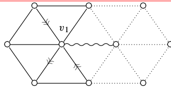
FIGURE 11. Case v_1 \in Z_{12}
