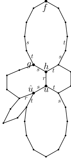
FIGURE 6. Proof of Proposition 5.1, Case 3.
