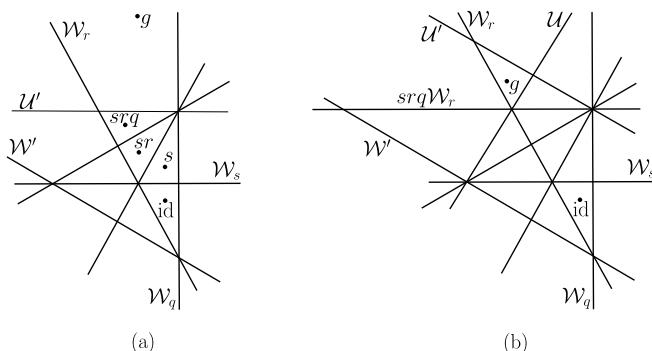
Fig. 2 Proof of Lemma 3.2, the case m_{sq} = 2 , m_{sr} = 3 , and W' = rW_q
