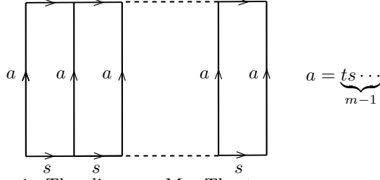
FIGURE 1. The diagram M . The top arrows are either all labelled s or all labelled t , depending on the parity of m .
