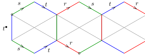
FIGURE 8. Dashed lines indicate possible polarisations.
