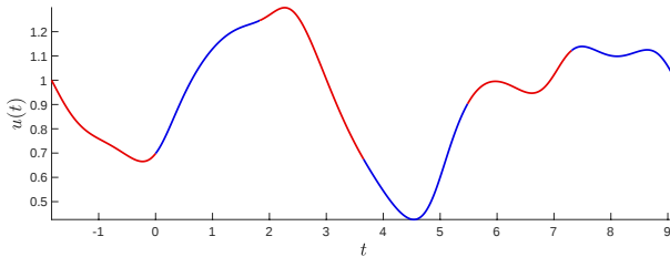
Figure 5: A rigorously validated 6-step periodic orbit in the Mackey-Glass equation at the parameter values \alpha = 2 , \beta = 1 and \rho = 9.65 . For the proof, we used N = 54 Chebyshev coefficients per component and fixed \nu = 1.05 . The radius enclosure of the orbit is given by r = 3.5 \times 10^{-8} and the delay \tau is given by the rigorous enclosure \tau \in 1.827334865 \pm [-r, r] . The code which performs the proof is script_proof_P0_Fig5_MG_period_6.m .
