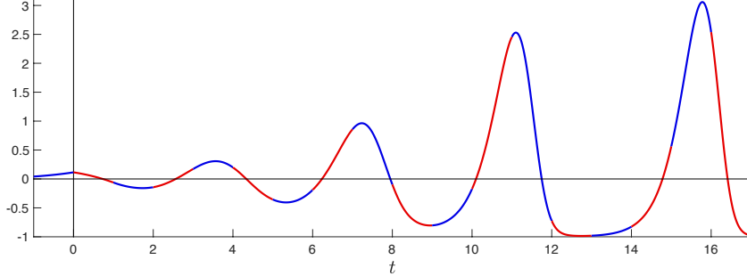
Figure 1: A rigorously computed 17-step orbit in Wright's equation at the parameter value \alpha \approx 2.350319657675625 . The final step appears to be close to an attracting periodic solution of Wright's. This illustrates an integration starting near an unstable equilibrium and terminating near the global attractor.
