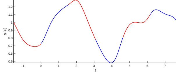
Figure 3: A rigorously validated 6-step periodic orbit of the Mackey-Glass equation at the parameter values \alpha = 2 , \beta = 1 and \rho = 10 . For the proof, we used N = 55 Chebyshev coefficients per component and fixed \nu = 1.05 . The radius enclosure of the orbit is given by r = 2.5 \times 10^{-8} and the delay \tau is given by the rigorous enclosure \tau \in 1.539575123 \pm [-r, r] . The code which performs the proof is script_proof_P0_Fig3_MG_period_6.m .
