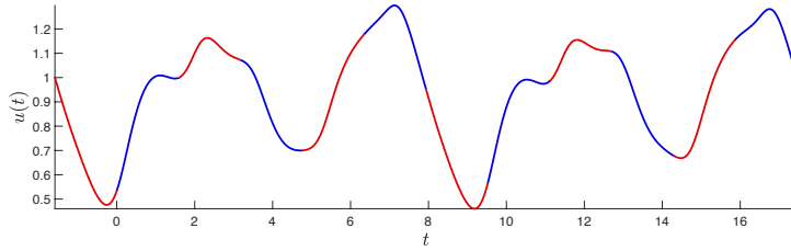
Figure 4: A rigorously validated 12-step periodic orbit in the Mackey-Glass equation at the parameter values \alpha = 2 , \beta = 1 and \rho = 10 . For the proof, we used N = 60 Chebyshev coefficients per component and fixed \nu = 1.033 . The radius enclosure of the orbit is given by r = 4.3 \times 10^{-8} and the delay \tau is given by the rigorous enclosure \tau \in 1.587078323 \pm [-r, r] . The code which performs the proof is script_proof_P0_Fig4_MG_period_12.m .
