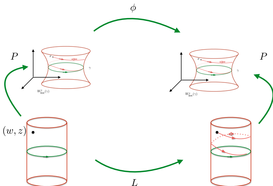
Fig. 1 Cartoon of the flow conjugacy Eq. (4) satisfied by solutions of Eq. (1)
