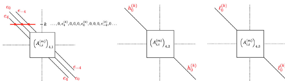
Fig. 7 Structure of the components of the operator A_{i,i} . The infinite dimensional diagonal and tridiagonal terms are defined so that the composition AA^{\dagger} acts as the identity out of \Pi^{(M+4)}X
