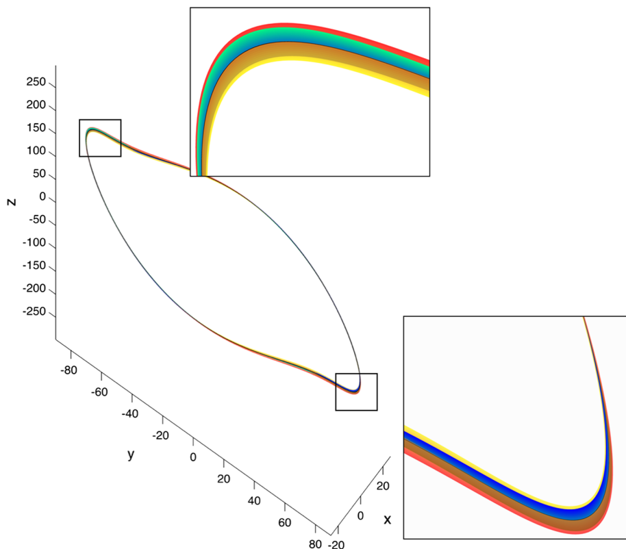
Fig. 5 Image of the parameterization of two submanifolds of the local stable manifold associated to the periodic orbit \Gamma(t) . Only the first three components of P_N(w, z) are drawn. The red-to-yellow surface is the image of the submanifold tangent to the eigenspace a_{(1,0)}(w) , associated to the Floquet exponent \lambda_1 \approx -7 . The green-to-blue surface is the submanifold tangent to the eigenspace a_{(0,1)}(w) , associated to \lambda_2 \approx -8 (Color figure online)
