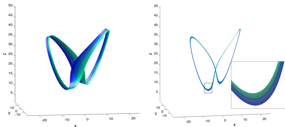
Fig. 3 Image of the local stable ( left ) and unstable ( right ) manifold associated to a periodic orbit of the Lorenz system at parameter \rho = 28
