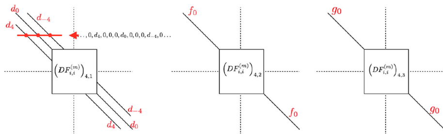
Fig. 6 Structure of the components of the operator A_{i,i}^{\dagger}
