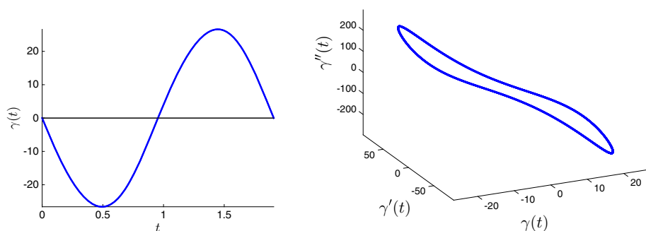
Fig. 4 (Left) The periodic solution \gamma(t) . (Right) The first three components of \Gamma(t) , periodic solution of the vector field (83)
