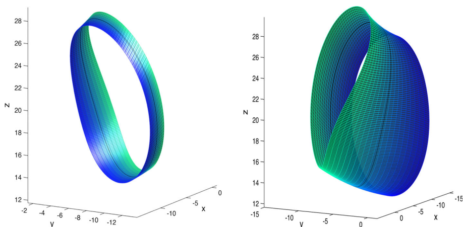
Fig. 2 Two images of the parameterization P_N(w, z) , |z| \leq v , N = 10 , of the local stable manifold associated to the periodic orbit of the Lorenz system at parameter \rho = 22 . In the left case v = 1 and the N -tail norm is \|H\|_{r,v}^\infty \leq 1.024 \cdot 10^{-11} . On the right v = 4 and \|H\|_{r,v}^\infty \leq 9.77 \cdot 10^{-5}
