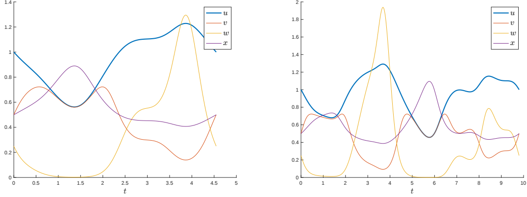
Figure 4: Two solutions of (44) for \tau = 1.63 , \rho = 10 , corresponding to solutions N°1 with \hat{\vartheta} = 1.3819 (left) and N°3 with \hat{\vartheta} = 0.6412 (right) from Table 1.
