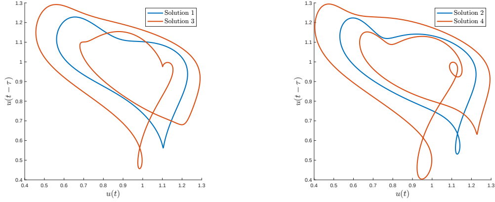
Figure 3: All four verified solutions plotted using delay embedding coordinates. Left: Solutions №1 and №3 from Table 1, corresponding to \tau = 1.63 . Right: Solutions №2 and №4 from Table 1, corresponding to \tau = 2 .
