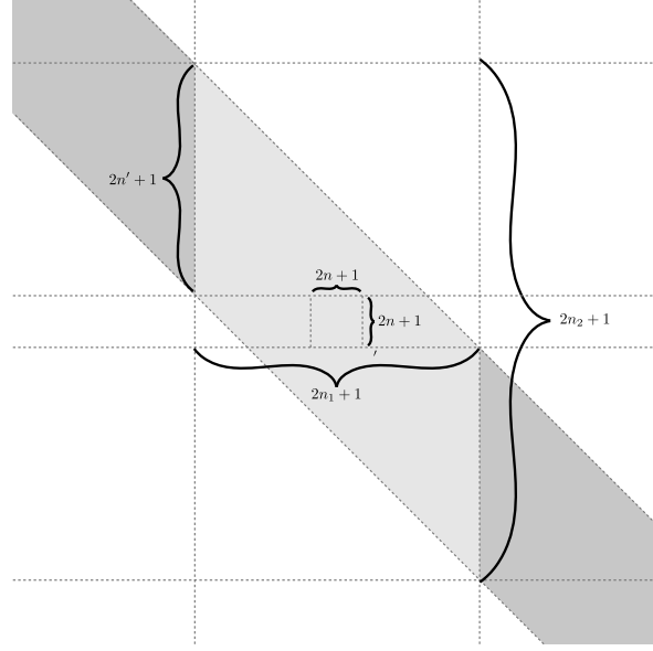
Figure 2: A sketch of the entries of the pseudo-convolution operator \Gamma_S(a) as a \mathbb{Z} \times \mathbb{Z} matrix. The light- and dark-grey part represents the nonzero entries of \Gamma_S(a) . The darker grey area represents the nonzero entries of the operator \pi^{n,\infty}\Gamma_S(a)\pi^{n_1,\infty} for a \in \mathbb{C}^{2n'+1} \subset \ell_\nu^1 with n < n' and n_1 = n + n' .
