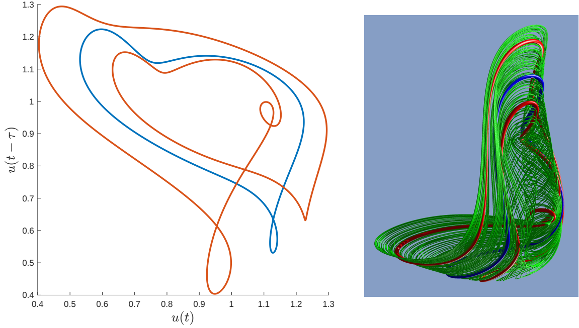
Figure 1: Two periodic solutions found in the chaotic regime, corresponding to \alpha = 2 , \beta = 1 , \tau = 2 and \rho = 9.65 . Left: a parametric plot of (u(t), u(t - \tau)) of the two solutions. Right: a 3-dimensional rendering of (u(t), u(t - \tau/2), u(t - \tau)) for the same two solutions. Also depicted is a (numerical) long orbit with random initial data, to illustrate the nature of the chaotic attractor.
