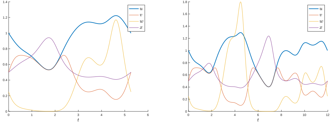
Figure 5: Two solutions of (44) for \tau = 2 , \rho = 9.65 , corresponding to solutions N°2 with \hat{\vartheta} = 1.1932 (left) and N°4 with \hat{\vartheta} = 0.5251 (right) from Table 1.
