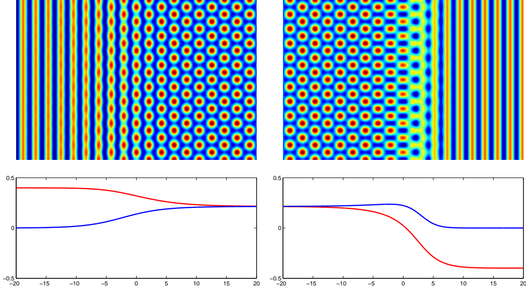
Figure 1: At the bottom are graphs of B_1 (red) and B_2 (blue) representing heteroclinic solutions of (1.2) that connect the hexagon state to the positive rolls (on the left) and negative rolls (and the right). The parameter values are \tilde{c} = 0 , \tilde{\mu} = \frac{7+3\sqrt{6}}{30} and \tilde{\beta} = 1 , corresponding to the assumptions in Theorem 1. At the top are the corresponding stationary patterns of (1.1). We note that the two phase transitions from rolls to hexagons have distinctive features. On the left, the stripes (“positive” rolls) undergo pearling, which gradually leads to separation into spots (hexagons). On the right, the stripes (“negative” rolls) develop transverse waves, which break up into a block structure that then transforms into hexagonal spots.
