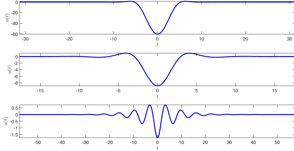
Figure 6: The solution profiles in the variable u of the suspension bridge equation (1.2) for \beta = 0.5 (top), \beta = 1.2 (middle) and \beta = 1.9 (bottom). Notice the different scales of the y -axis for the three solutions.
