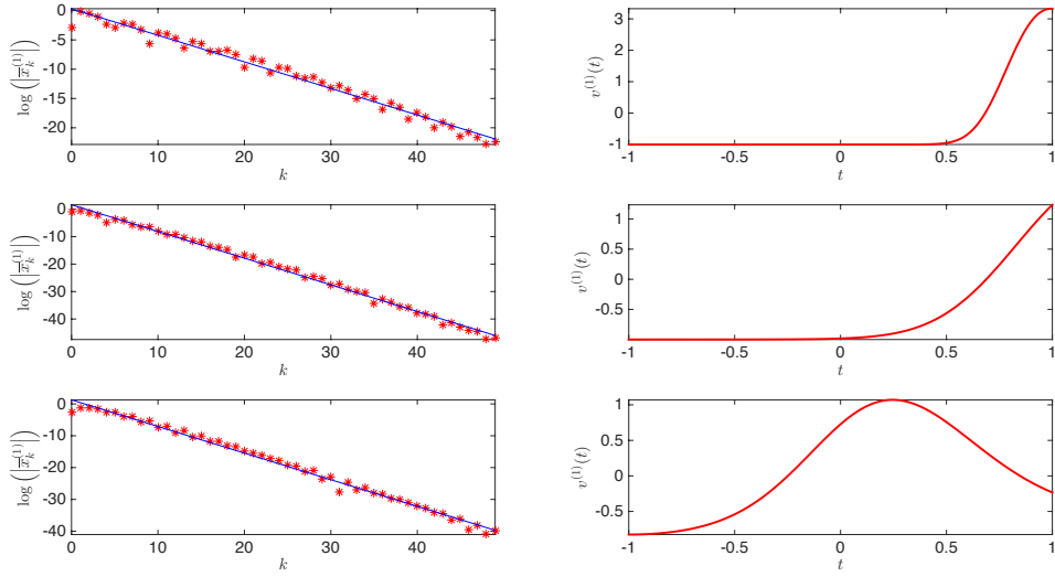
Figure 1: The logarithm of the absolute value of the 50 first coefficients of the first component on the left, and the profile of the first component of the solution on the right. At the top \beta = 0.5 , in the middle \beta = 1.2 and at the bottom \beta = 1.9
