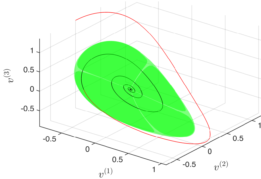
Figure 4: First three components of the solution (red) and the manifold (green) in the case \beta = 1.9 . The segment in black corresponds to the forward orbit of the solution on the local manifold, where the dynamics is obtained via the conjugacy relation satisfied by the parameterization.
