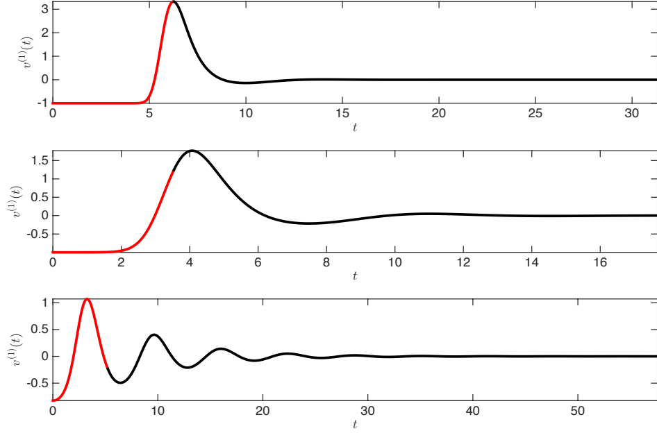
Figure 5: The solution profiles of v^{(1)}(t) for \beta = 0.5 (top), \beta = 1.2 (middle) and \beta = 1.9 (bottom). The parts in red correspond to the part of the solution which was obtained using Chebyshev series, while the parts in black correspond to the part of the solution lying in the local stable manifold computed using Taylor series.
