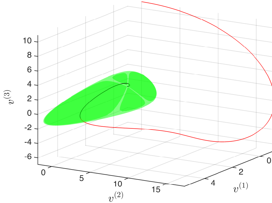
Figure 2: First three components of the solution (red) and the manifold (green) in the case \beta = 0.5 . The segment in black corresponds to the forward orbit of the solution on the local manifold, where the dynamics is obtained via the conjugacy relation satisfied by the parameterization (e.g. see [7]).
