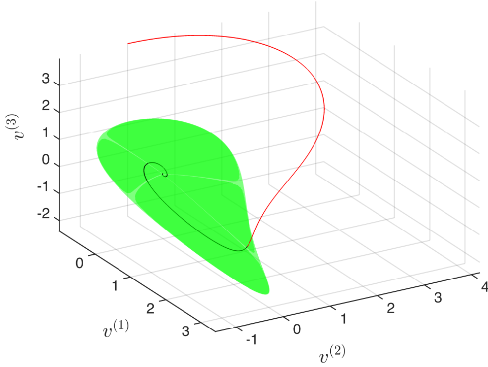
Figure 3: First three components of the solution (red) and the manifold (green) in the case \beta = 1.2 . The segment in black corresponds to the forward orbit of the solution on the local manifold, where the dynamics is obtained via the conjugacy relation satisfied by the parameterization.
