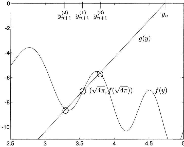
FIG. 1. Graph of f(y) and g(y) against y with multiple solutions indicated.
