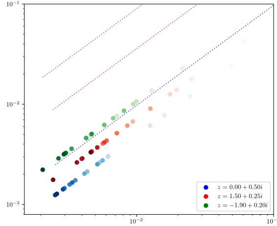
Figure 3: Convergence and boundedness of |\hat{\delta}_N| in relation to |\hat{\varepsilon}_N| on a log-log scale. Dotted lines represent bounds. Opacity of points increases as N increases.
