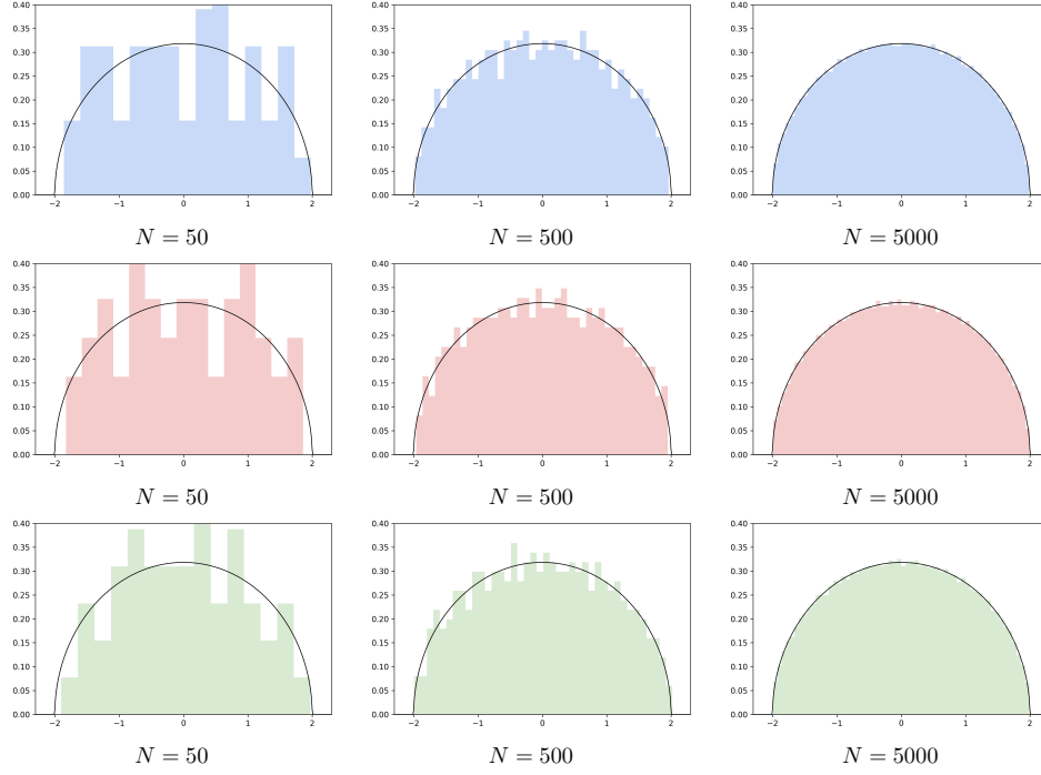
Figure 1: Convergence of \hat{\rho} to the semicircle law.
