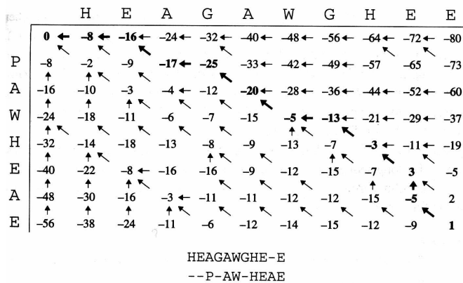
Figure 5: The optimal global alignment.
