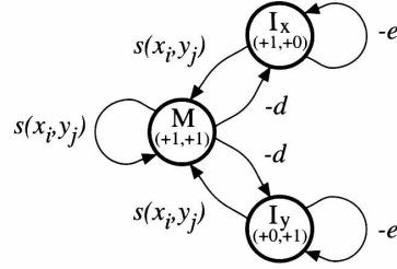
Figure 6: A diagram of the gapped alignment algorithm
