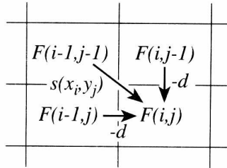
Figure 4: Recursive calculation of the F matrix
