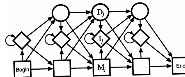
Figure 12: Chain with delete states
