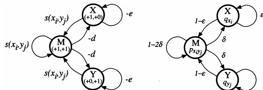
Figure 10: Chain for alignment
