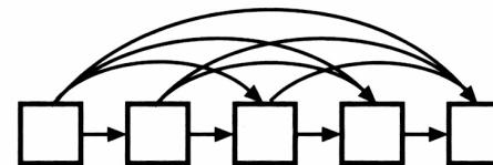
Figure 8: Chain without Silent States
