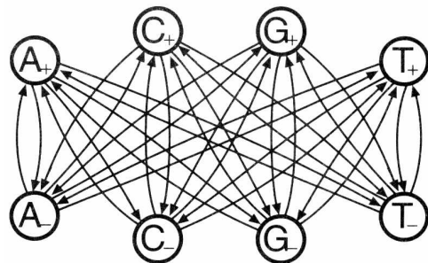
Figure 7: State model for CpG island HMM
