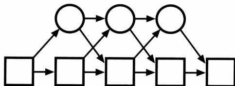
Figure 9: Chain with Silent States
