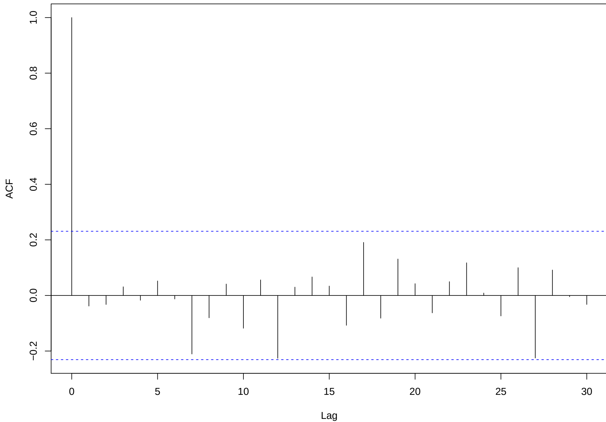
Series as.numeric(resid(f2))
