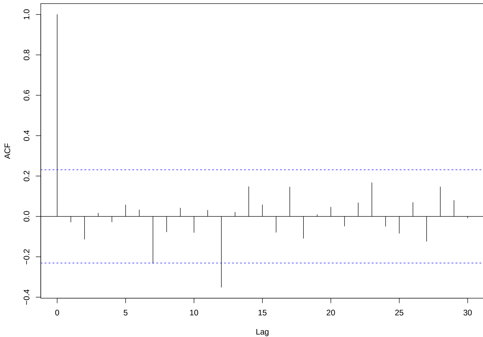
Series as.numeric(resid(f1))
