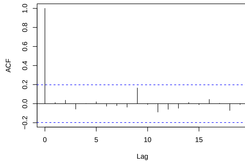
ARMA(1,1) residuals
