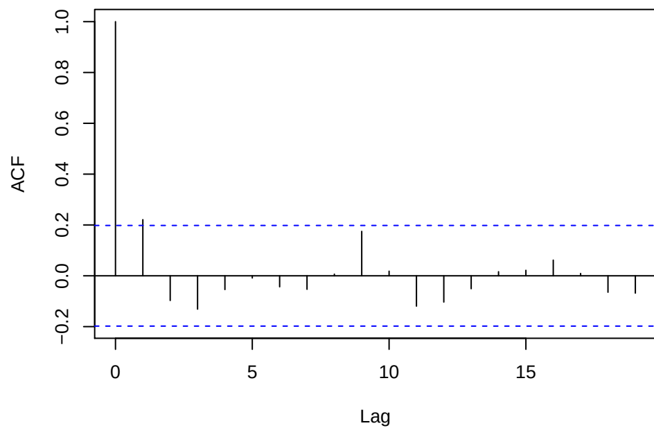
MA(1) residuals
