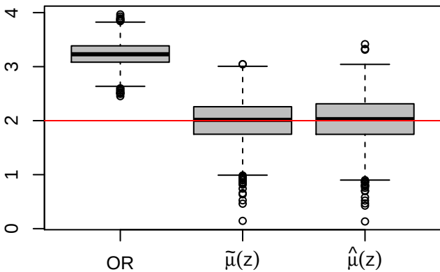
\mu(0, 0)
