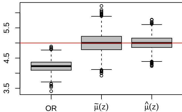
\mu(1, 0)
