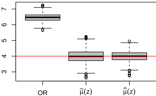
\mu(0, 1)
