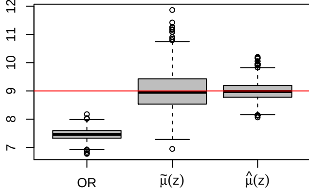
\mu(1, 1)
