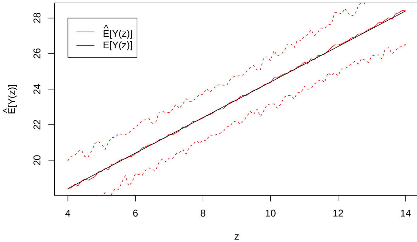
\hat{E}[Y(z)] with stabilized weight
