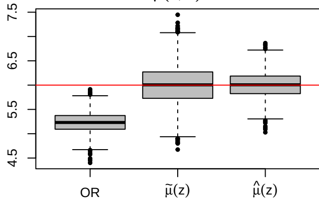
\mu(1, 0)
