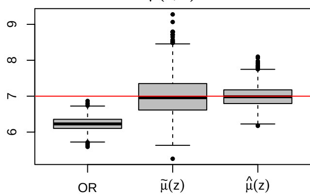
\mu(1, 1)
