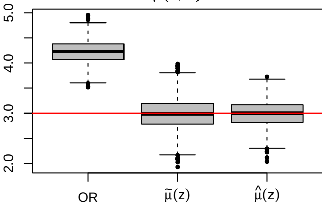
\mu(0, 1)
