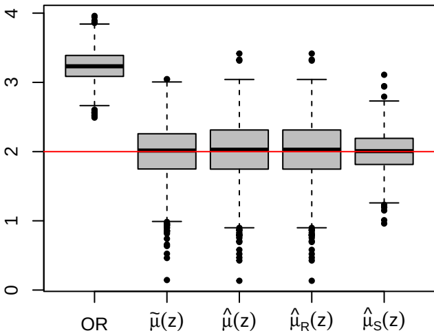
\mu(0, 0)
