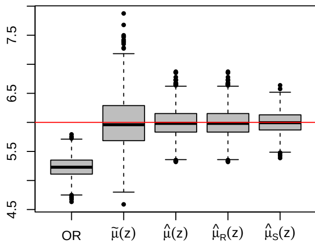
\mu(1, 1)
