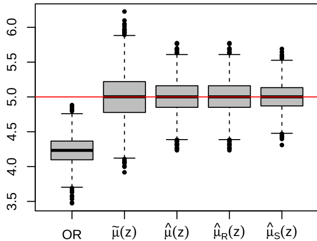
\mu(1, 0)
