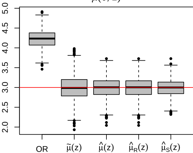
\mu(0, 1)
