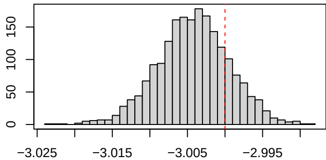
\Psi_3
