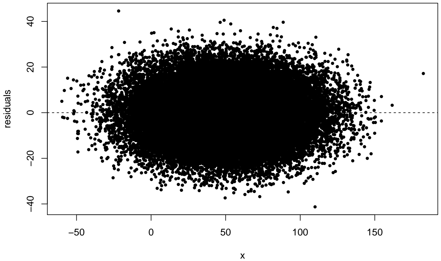
Larger sample size (50000) Straight line assumption correct
