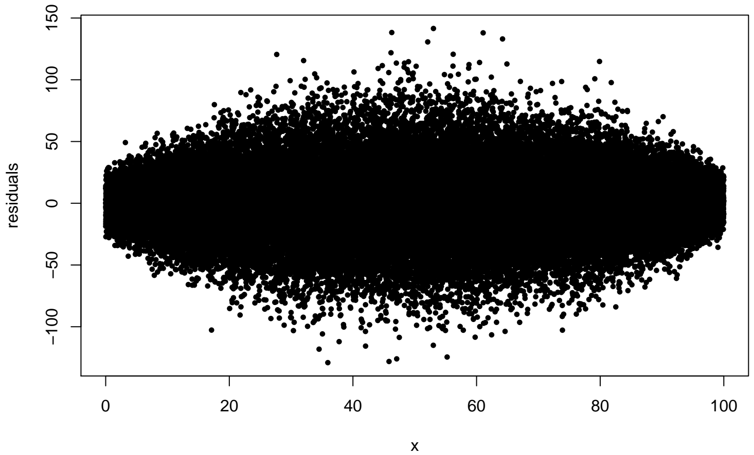
Larger sample size (50000) Incorrect constant variance assumption
