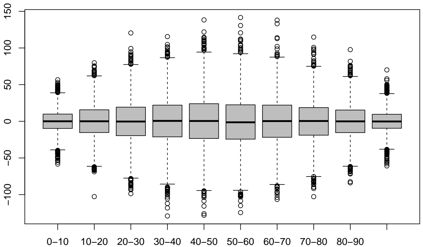
Residuals show non-constant variance pattern in boxplot
