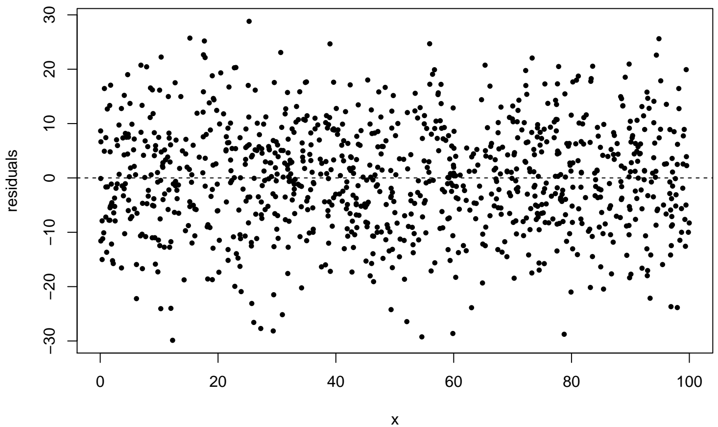
Residuals show no pattern vs x Straight line assumption correct
