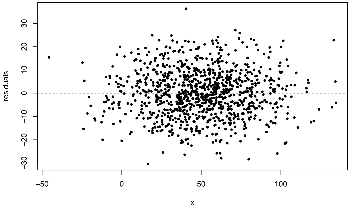
Residuals show no pattern vs x Straight line assumption correct
