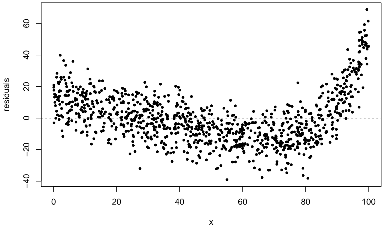
Residuals show curvilinear pattern vs x Incorrect straight line assumption
