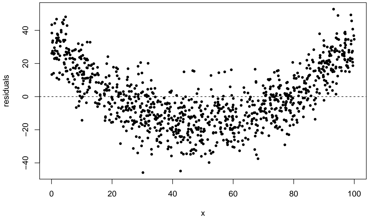
Residuals show parabolic pattern vs x Incorrect straight line assumption
