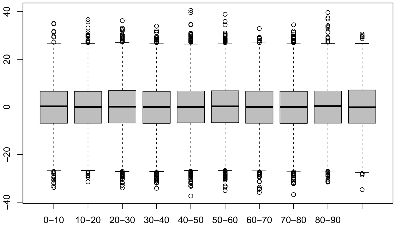
Residuals show constant variance pattern in boxplot
