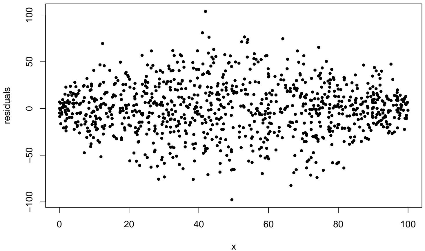
Residuals show non-constant variance pattern vs x Incorrect constant variance assumption
