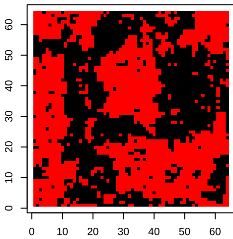
Gibbs Iteration 50
