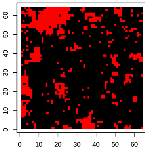
SW Iteration 30
