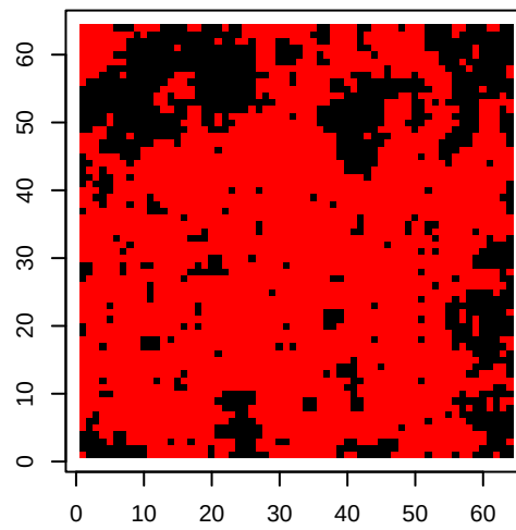
SW Iteration 40
