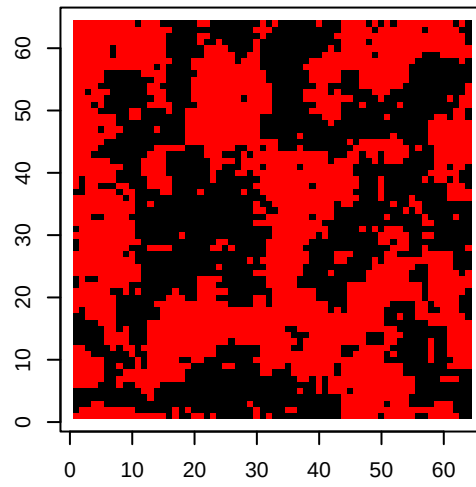
Gibbs Iteration 20
