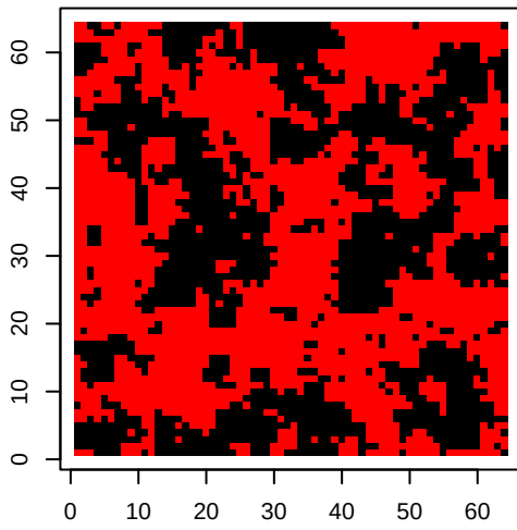
Gibbs Iteration 10
