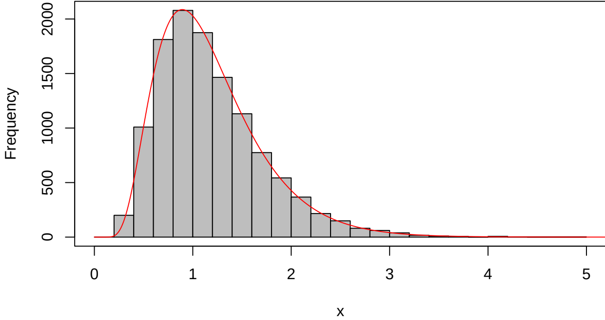
Histogram of Rejection sampling samples for X
