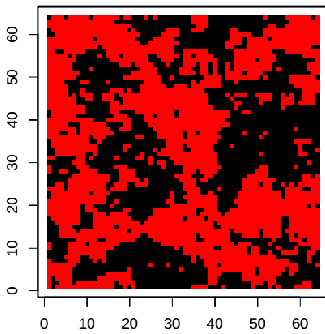
Gibbs Iteration 30
