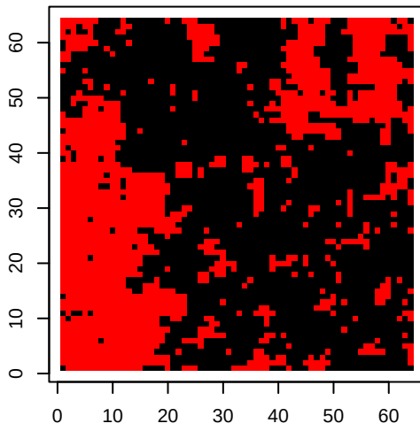
SW Iteration 10
