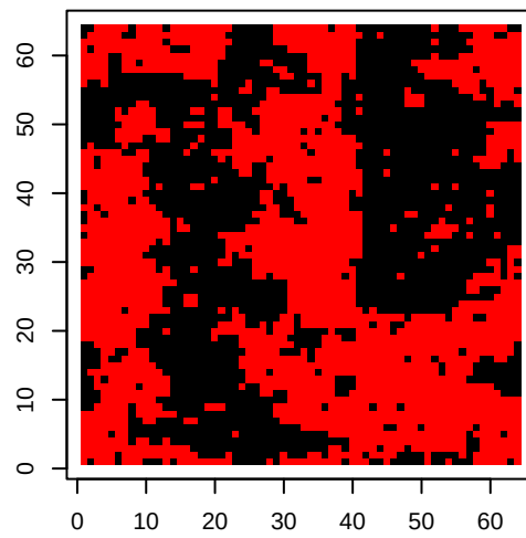
Gibbs Iteration 60
