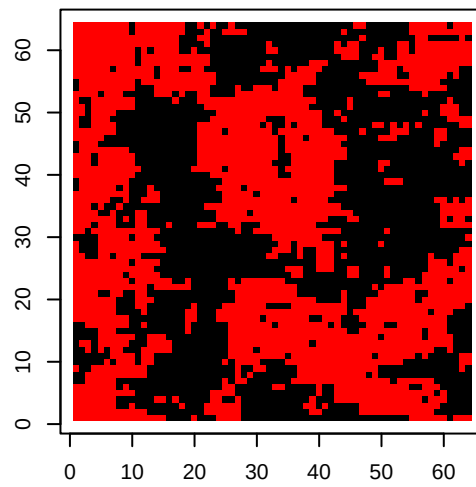
Gibbs Iteration 40
