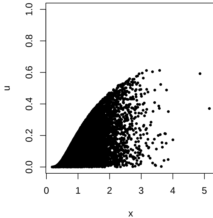
Sample from joint pdf of (X,U)
