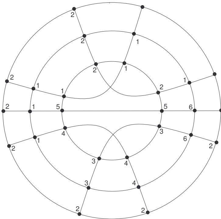
Figure 7: A separated doublecross giving rise to a K_6 minor.
