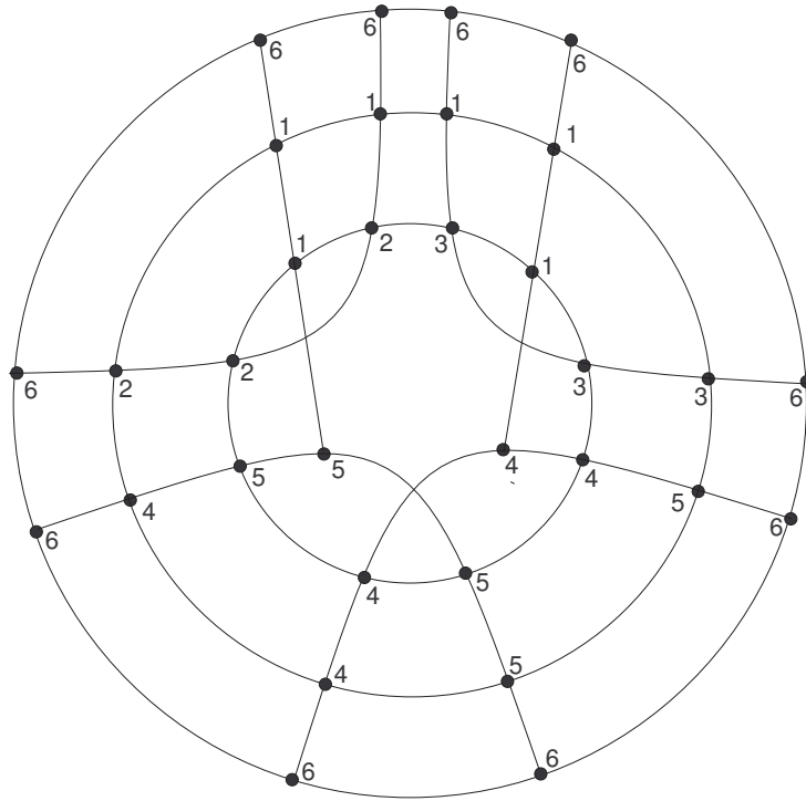
Figure 4: A turtle giving rise to a K_6 minor.
