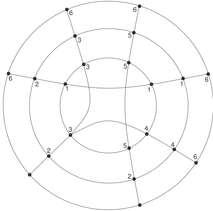
Figure 6: A gridlet giving rise to a K_6 minor.
