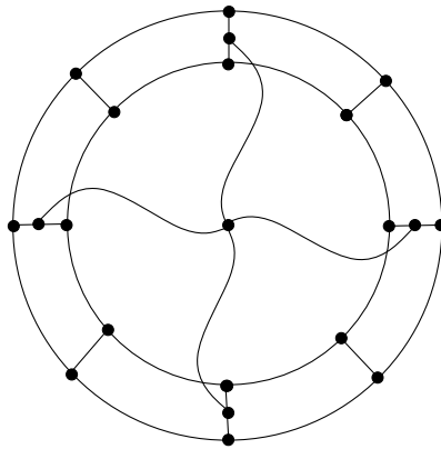
Figure 2: A pinwheel with four vanes.
