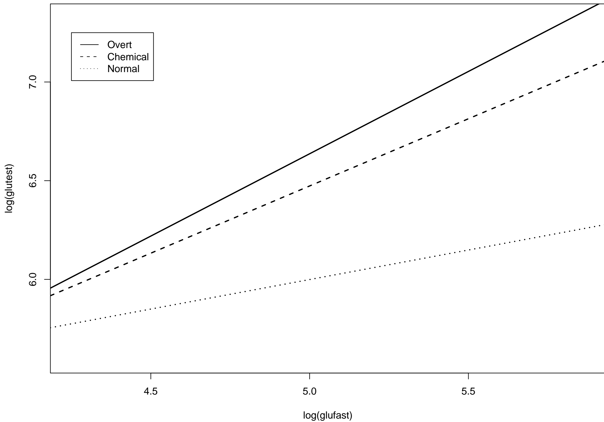
Fits to the three subgroups
