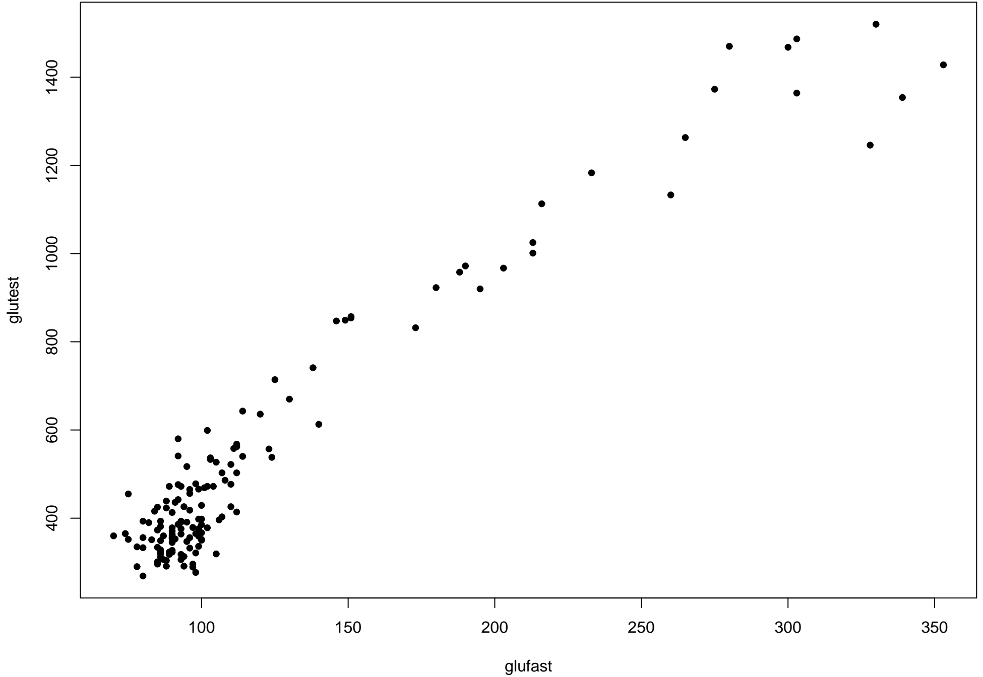
Original Data
