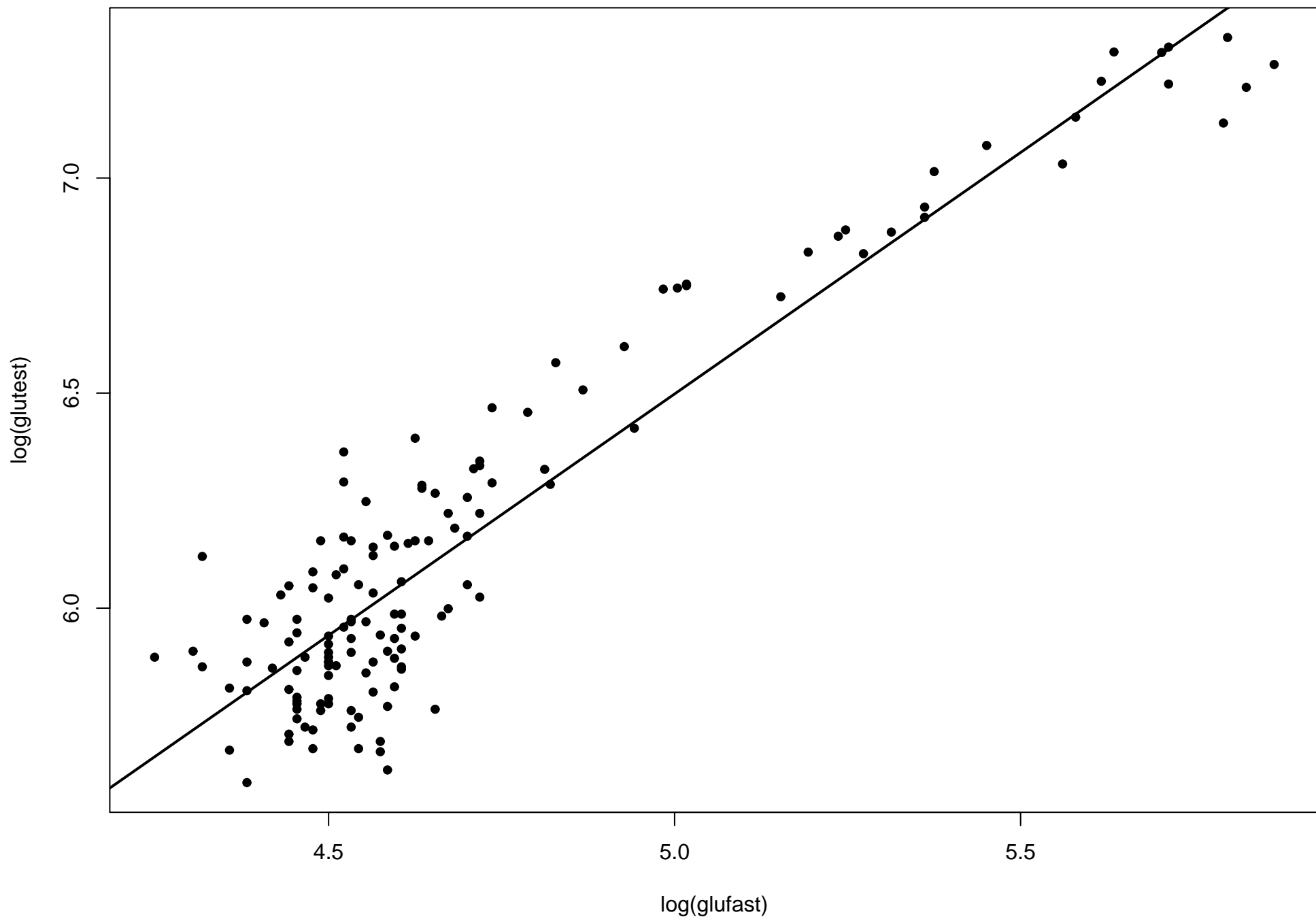
Log-scale Data
