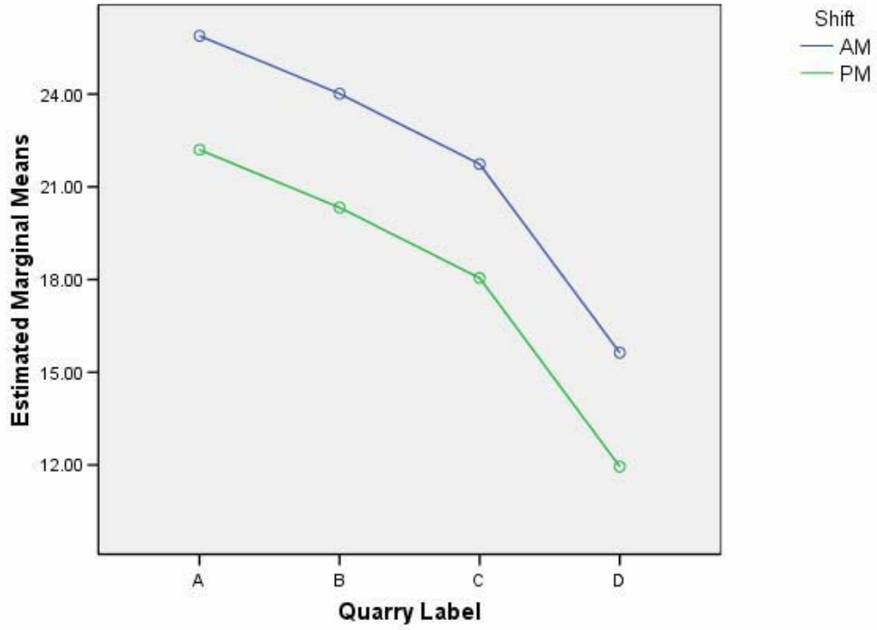
Estimated Marginal Means of amount
