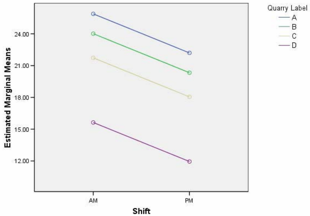
Estimated Marginal Means of amount
