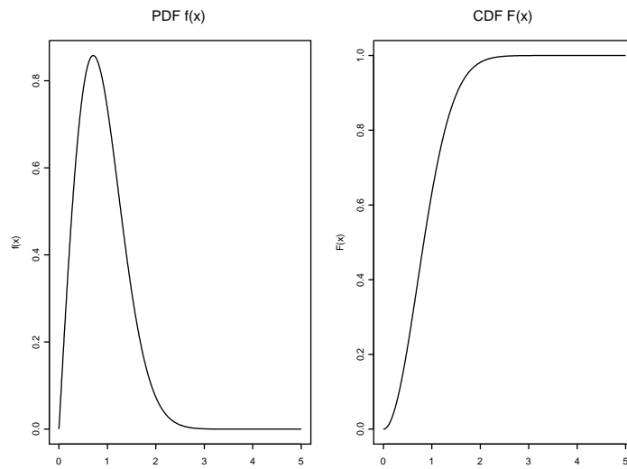
Figure 4: PDF f_X(x) = 2x \exp\{-x^2\} , x > 0 , and CDF F_X(x) = 1 - \exp\{-x^2\} , x > 0
