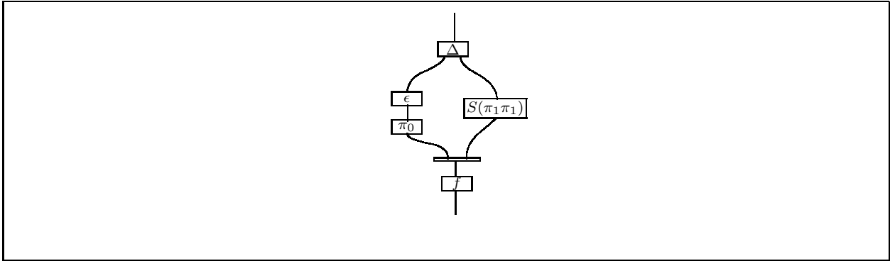
Figure 3: (\mathbf{1} \times \pi)D_{\times}[f] in \mathbb{X}
