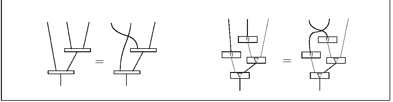
Figure 6: 1 \otimes d_{\otimes}; d_{\otimes} = c \otimes 1; 1 \otimes d_{\otimes}; d_{\otimes}
