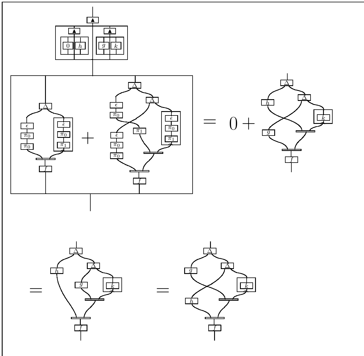
Figure 7: \langle\langle 0, h \rangle, \langle g, k \rangle\rangle D_{\times}[D_{\times}[f]]
