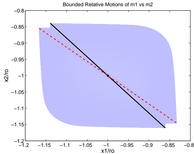
Figure 9. A solution (plotted in grey) of the forward surrogate dynamical system with \chi = 0 , m_1 = 1 , m_2 = 2 , r_o = 10^3 , \varepsilon_o = 2.5 \times 10^{-7} , \kappa = 2 , and \alpha = 6.2502 \times 10^3 . The periodic solution of the linearized equation (9) with \sigma = 2.5 , period T = 5.0265 \times 10^3 and A_1 = 0.13901 , A_2 = -0.16028 (shown in black) is used as the initial history for the solution of the nonlinear equation (2) which is plotted over a time interval of 600T .
