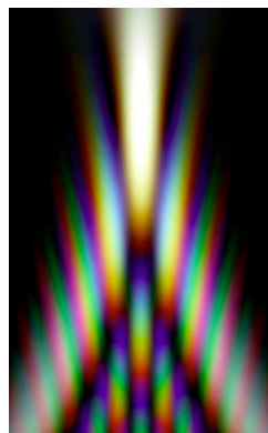
Cusp diffraction .
