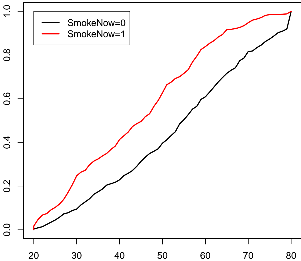
Cumulative distribution of Age by treatment group
