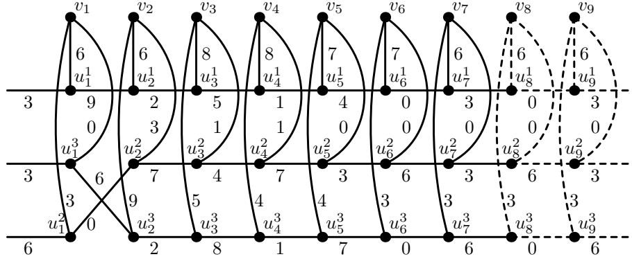
Figure 1: The construction of a 10/3 -circular edge-coloring of large flower snarks. The colors of the edges are multiplied by three in the figure.
