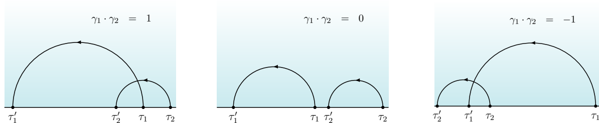
FIGURE 1. The topological intersection number \gamma_1 \cdot \gamma_2
